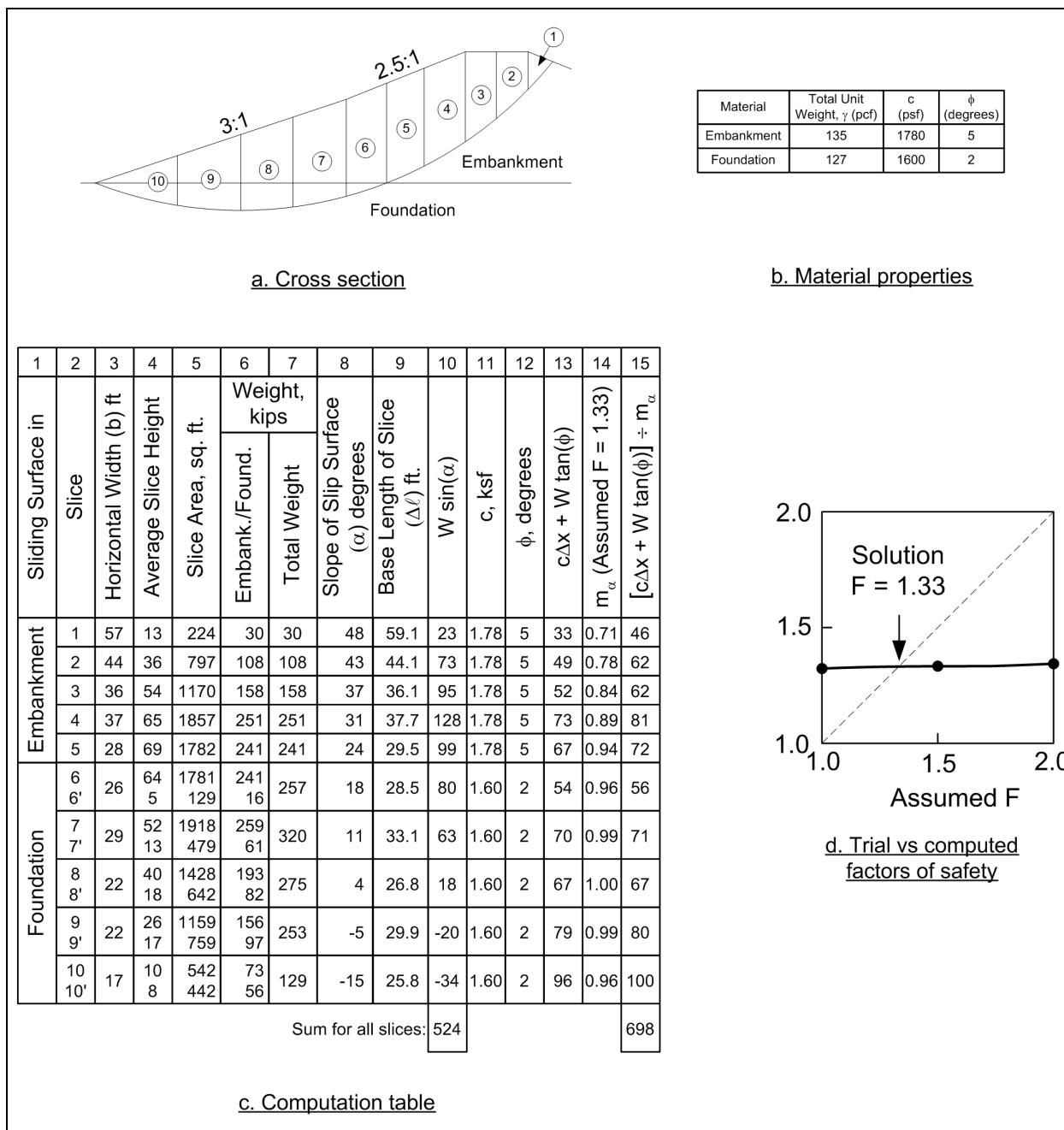
Figure F-11. End-of-construction example – Simplified Bishop Method
