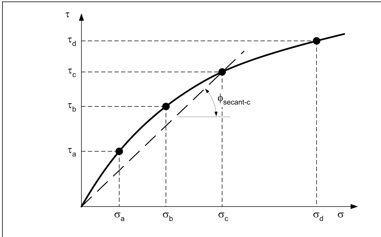
Figure D-17. Construction of curved strength envelope using secant friction angles
