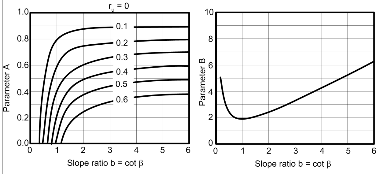
Figure E-7. Slope stability charts for infinite slopes (after Duncan, Buchianani, and DeWet 1987)
